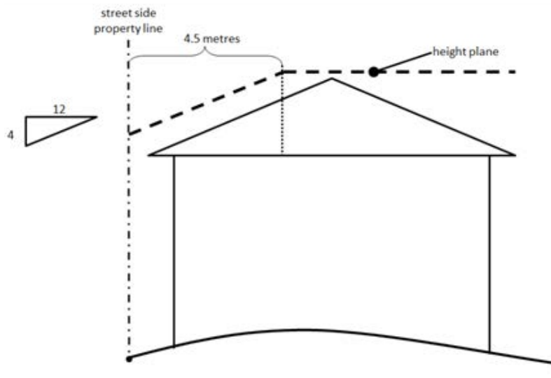
Building Height on a Corner Parcel Section 361(1)
