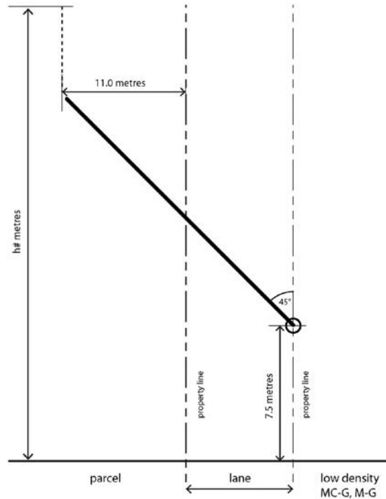
1381 (4) Building Height
